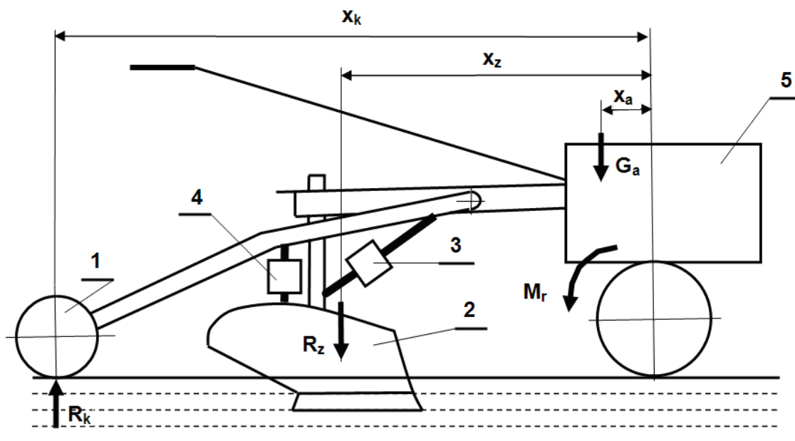
Fig.1. The diagram of the aggregate: 1 - support wheel, 2 - plow body, 3 and 4 - tensometric sensors, 5- moto block.
