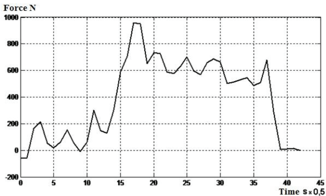
Fig.2. The graph of the traction force
