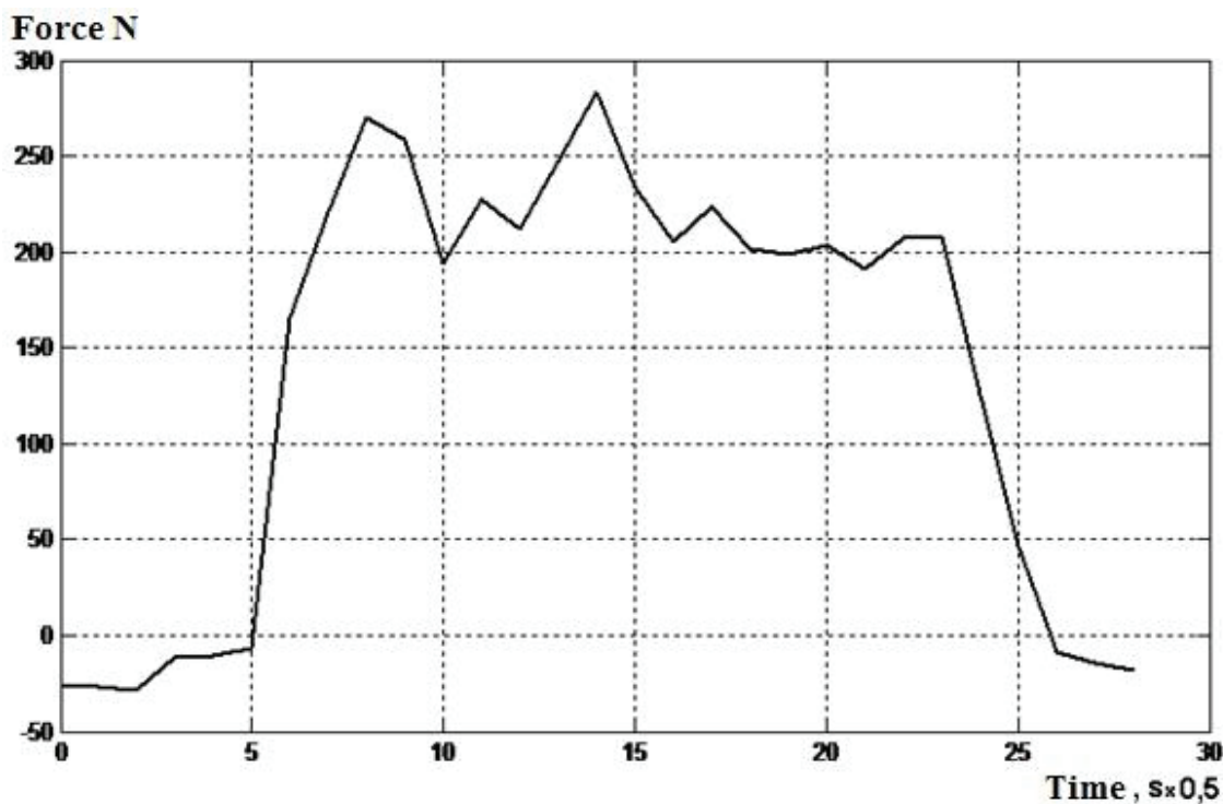
Fig.3. The graph of the force R_k in the support wheel
