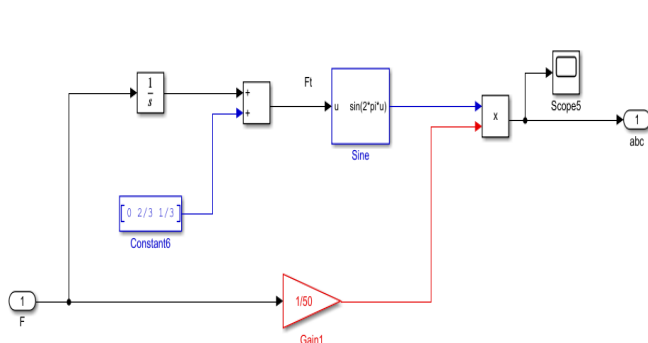
Fig.3. Block for V/f control of induction motor
