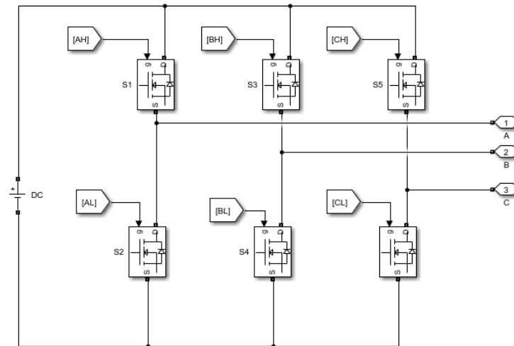
Fig.5. Inverter block
